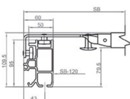
Profil SLIMLINER Small Profile SLIMLINER Small
