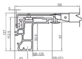
Profil SLIMLINER Medium Profile SLIMLINER Medium
