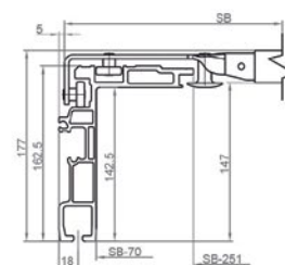
Profil SLIMLINER Large Profile SLIMLINER Large
